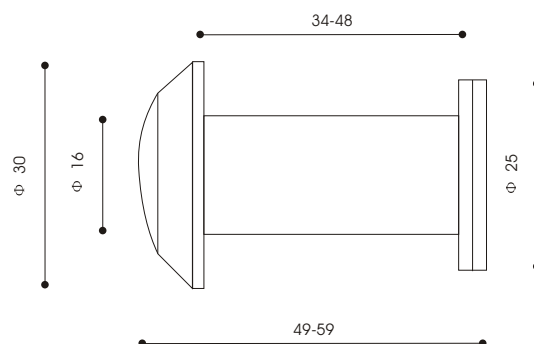
Brass door viewer/貓眼(銅)
