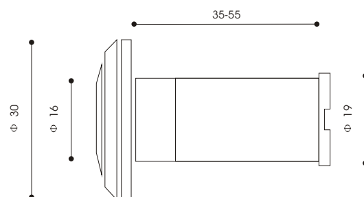
Brass door viewer/貓眼(銅)
