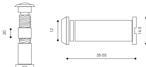
Brass door viewer/貓眼(銅)
