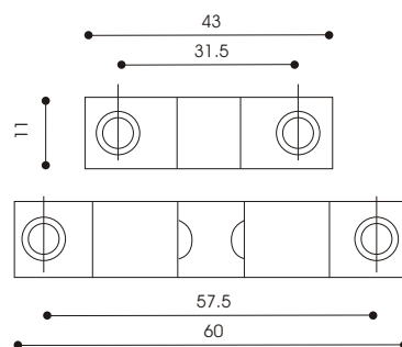
Brass double ball catch / 雙碰珠(銅)
