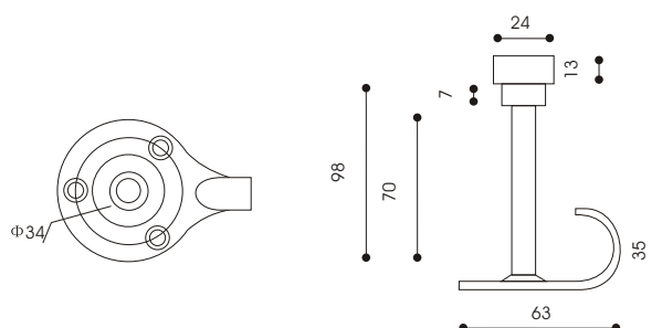
Stain steel door stopper/門碰(不銹鋼)
