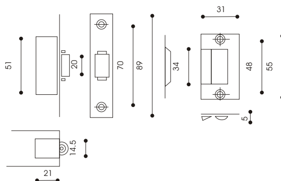
Stain steel dust ball catch / 碰珠(不銹鋼)
