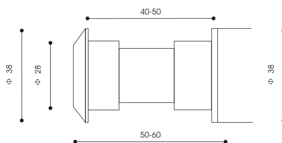
Brass door viewer/貓眼(銅)
