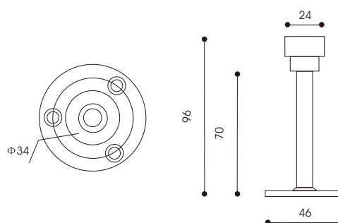
Stain steel door stopper/門碰(不銹鋼)
