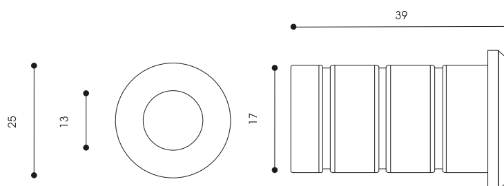
Stain steel dust proof strike/防塵筒(不銹鋼)
