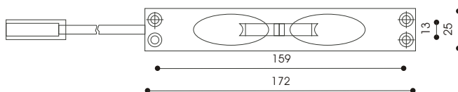
Brass door bolt/插銷(銅)
