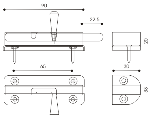
Stain steel door bolt/插銷(不銹鋼)
