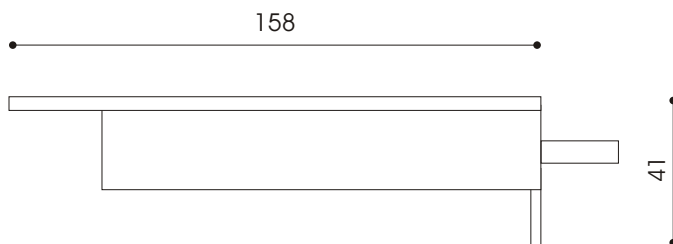
Stain steel door bolt/插銷(不銹鋼)
