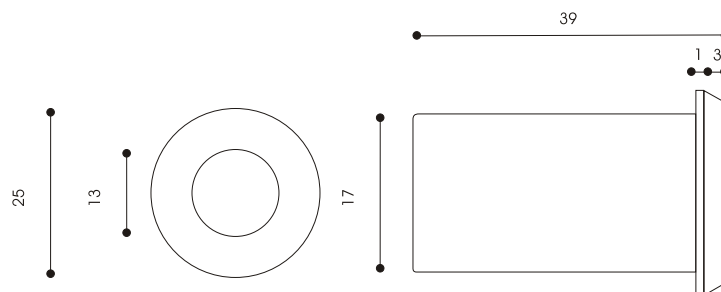
Brass dust proof strike/防塵筒(銅)
