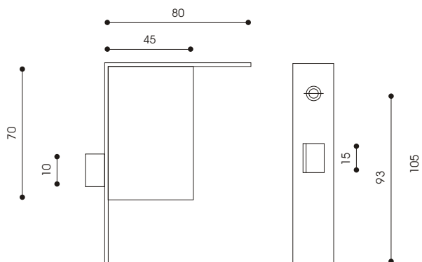
Stain steel door bolt/插銷(不銹鋼)
